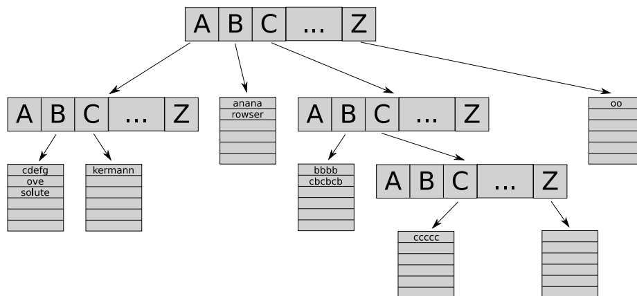
Figure G.1: Burstersort data structure
